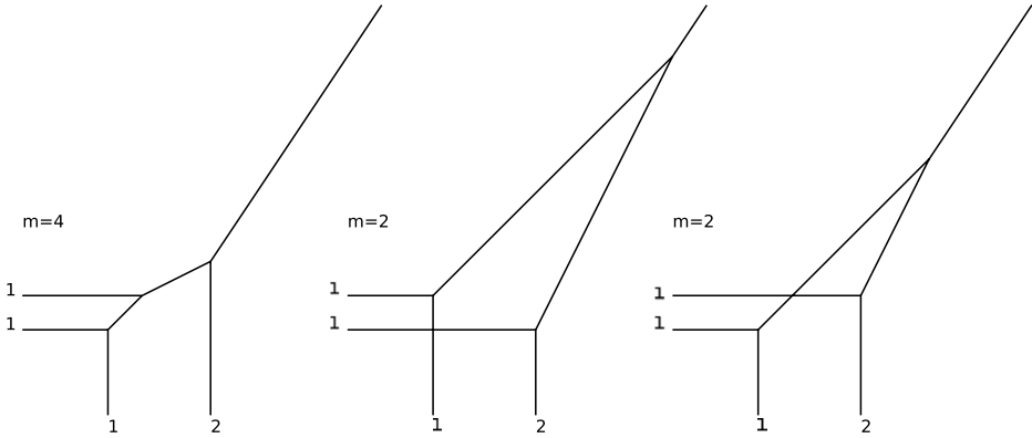
Fig. 1. N^{\text{trop}}(1 + 1, 1 + 2) = 8 .
