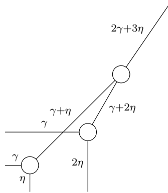
FIGURE 4. The tropical type C_2
