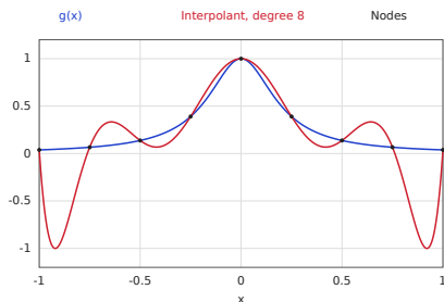
Degree 8: 9 equally spaced nodes
