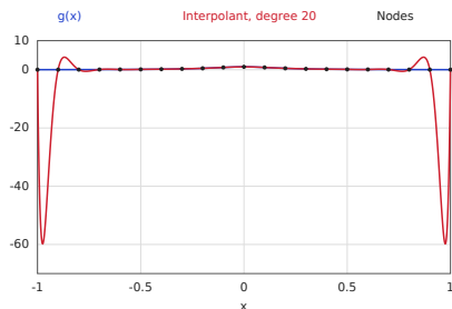
Degree 20: 21 equally spaced nodes
