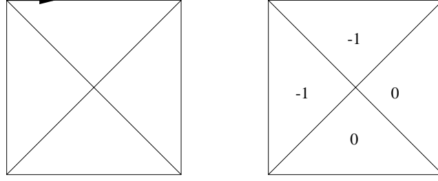
FIGURE 6. The divergence of an element in \Sigma_h
