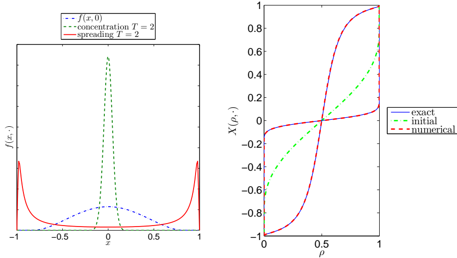
FIG. 7.1. Benchmark case: evolution of density function (left hand side figure) and comparison between analytical and numerical solution for the quantile function (right hand side figure)
