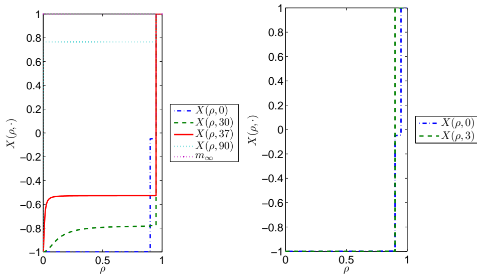
FIG. 7.4. Plot of the behavior of a numerical “controversial” solution: concentration case tends to \delta_1 (left hand side figure), while 1 - 2\epsilon mass goes to -1 in the spreading case (right hand side figure)
