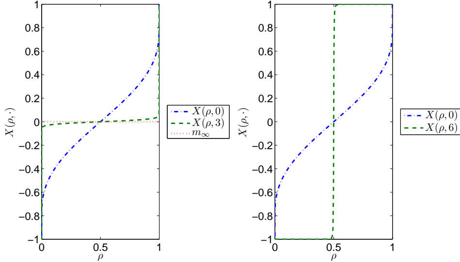
FIG. 7.2. Plot of the behavior of numerical solution with symmetric initial data for concentration case (left hand side figure), and for spreading case (right hand side figure)
