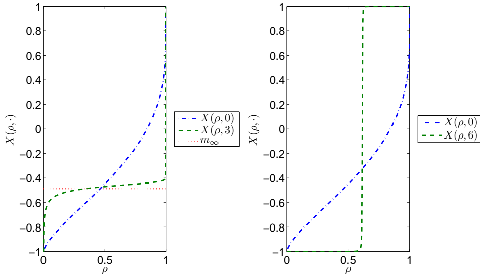
FIG. 7.3. Plot of the behavior of numerical solution with non symmetric initial data for concentration case (left hand side figure), and for spreading case (right hand side figure)
