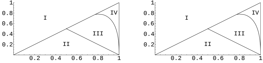
Figure 1: Left Regions for the parameter \mu and saving rate \lambda in Example 2. Pareto Tails are found in zone III. Right Critical value of the saving rate \lambda in Example 4. Pareto tails form for \lambda lying below the curve.
